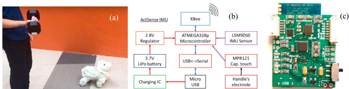
Fig. 7. Interaction between the hand motion through the dumbbell and SNOWY movements (a). Block diagram (b) and the Printed Circuit Board (PCB) (c) of the ActSense IMU board – the core of the interactive dumbbell
