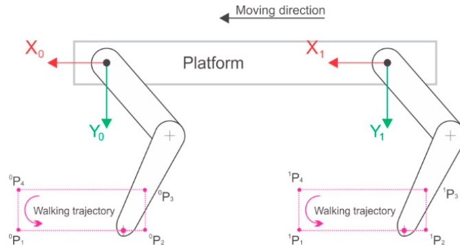
Fig. 5. Rectangular shape trajectory was chosen as walking trajectory for its simplicity.
