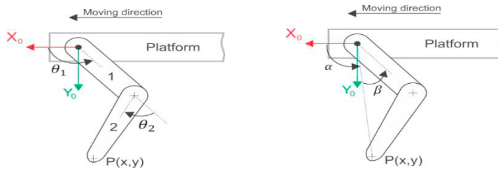
Fig. 4. Frame allocation of the simplified model of the leg with notations for different joint angles
