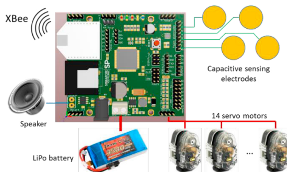
Fig. 2. Control system architecture of SNOWY
