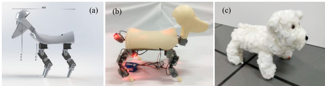
Fig. 1. Mechanical hardware design of the robot platform.-CAD design (a) bare mechanical frame without cover (b) and with soft fur covers (c) of the platform. The cover can be easily removable for washing and cleaning.
