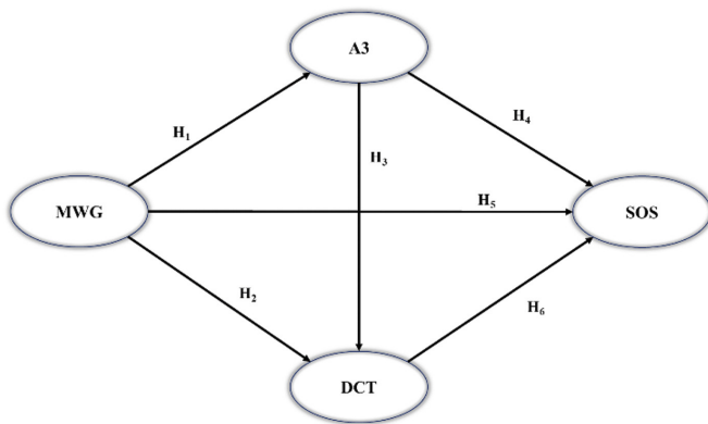
Fig 1. Proposed model
