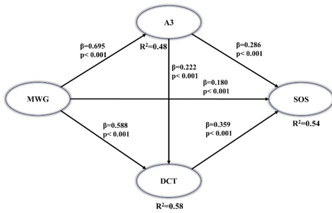
Fig 2. Evaluated model
