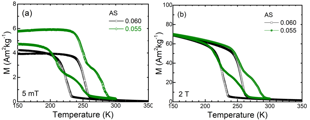
FIG. S2. Comparison of the ZFC and FC M(T)^{5mT} (a) and M(T)^{2T} (b) for as-solidified (AS) Mn_{0.5}Fe_{0.5}NiSi_{1-x}Al_x ribbon samples with x = 0.060 and 0.055 .
