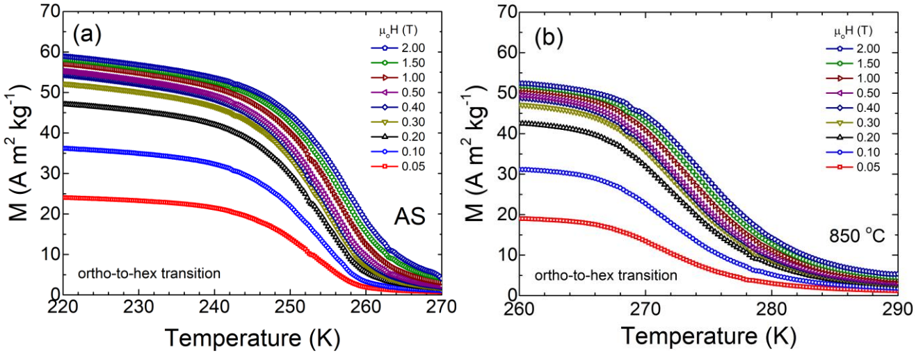
FIG. S3. Mn_{0.5}Fe_{0.5}NiSi_{0.940}Al_{0.060} ribbons: isofield M(T) curves measured on heating at selected static magnetic field values through the ortho-to-hex transition for as-solidified (a) and 850\text{ }^\circ\text{C} annealed (b) samples.
