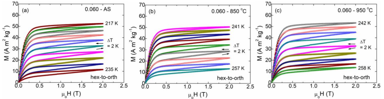
FIG. S4. Set of isothermal M(\mu_0H) curves measured through the hex-to-orth transition for as-solidified (a), 850\text{ }^\circ\text{C} (b) and 950\text{ }^\circ\text{C} (c) annealed ribbons with x = 0.060 from which the thermal dependence of the magnetic hysteresis losses HL(T) were obtained under its \delta T_{FWHM} temperature span.
