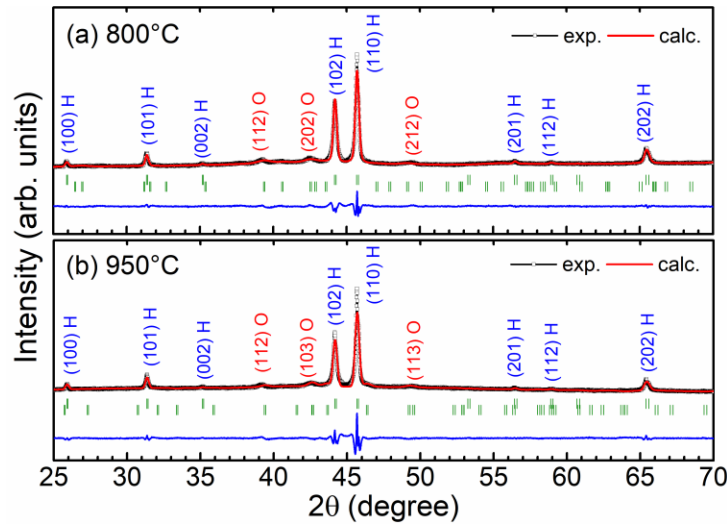
FIG. S1. Room temperature XRD pattern for the 800 °C (a) and 950 °C (b) annealed ribbons with x=0.060 .
