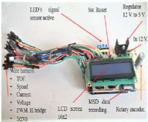
Figure 5. Arduino shield PCB interconnecting sensors, displays and actuators with the microprocessor.
