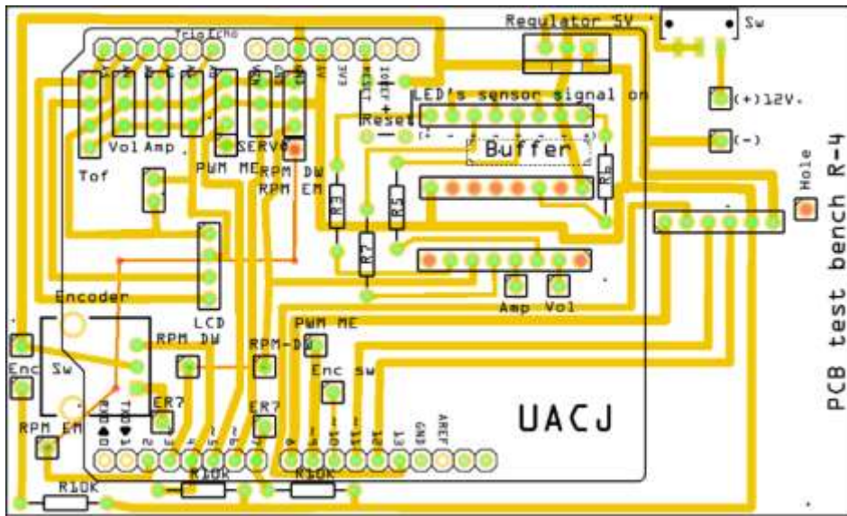
Figure 4. Arduino shield PCB interconnecting sensors, displays and actuators with the microprocessor.
