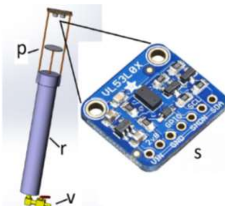
Figure 6. Sensor to measure fuel consumption using the VL53L0X module. A PCV reservoir (r) contains a float connected to a plate (p) through a dipstick. The VL53L0X emits a laser pulse to this plate, and it measures the TOF inferring the distance. This information is proportional to fuel amount in the reservoir.
