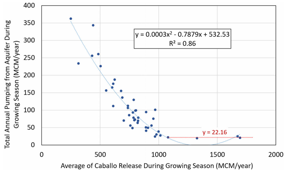
FIGURE 6. Regression relationship between total annual groundwater pumping and releases from Caballo Reservoir during the growing season.
