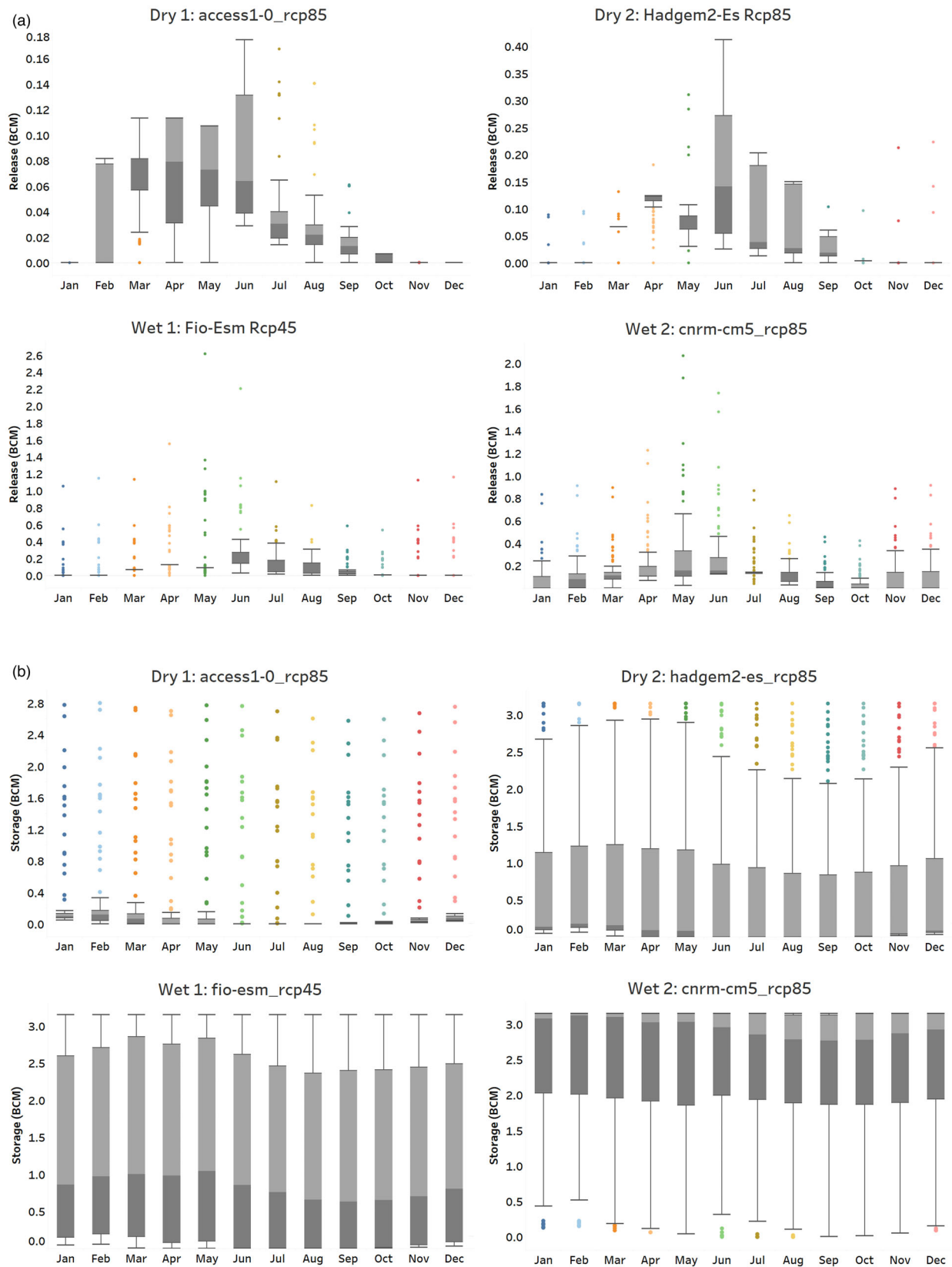
FIGURE 10. Ranges of Elephant Butte-Caballo reservoir system release (a) and storage (b) under selected climate-based flow scenarios through year 2099.
