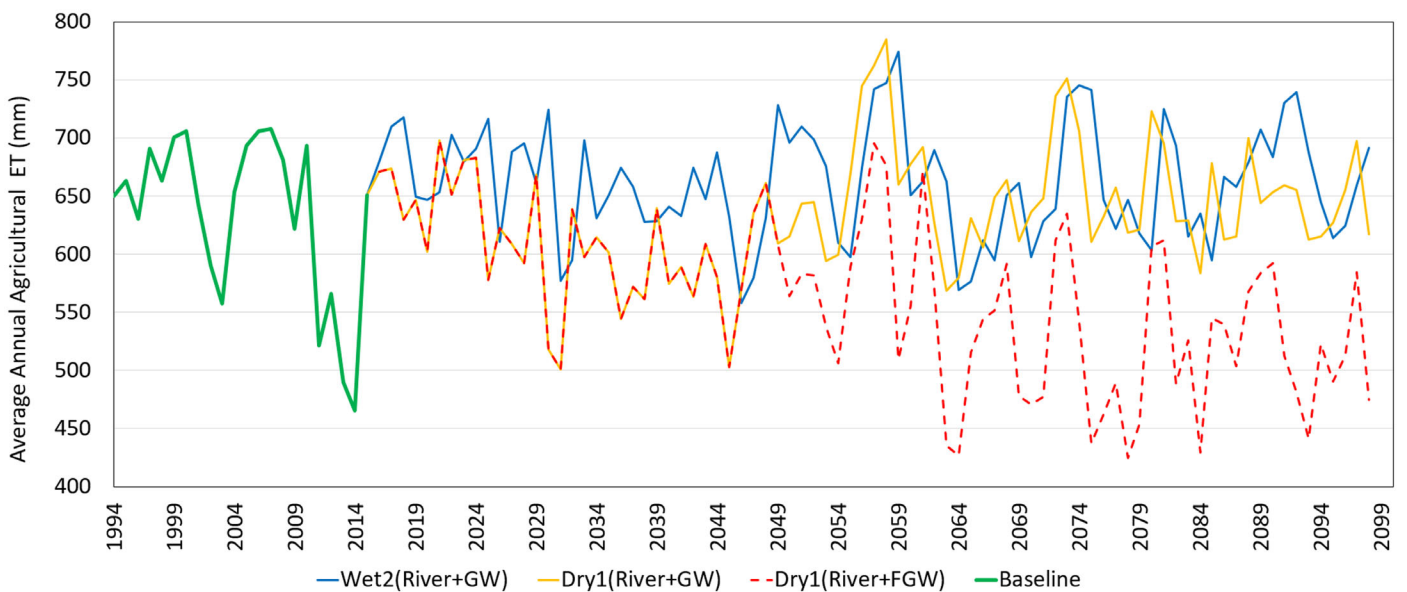
FIGURE 12. Simulated evapotranspiration for baseline, Wet2 and Dry 1 with all available water resources (River+GW) and Dry1 with surface water and fresh groundwater only (River+FGW).
