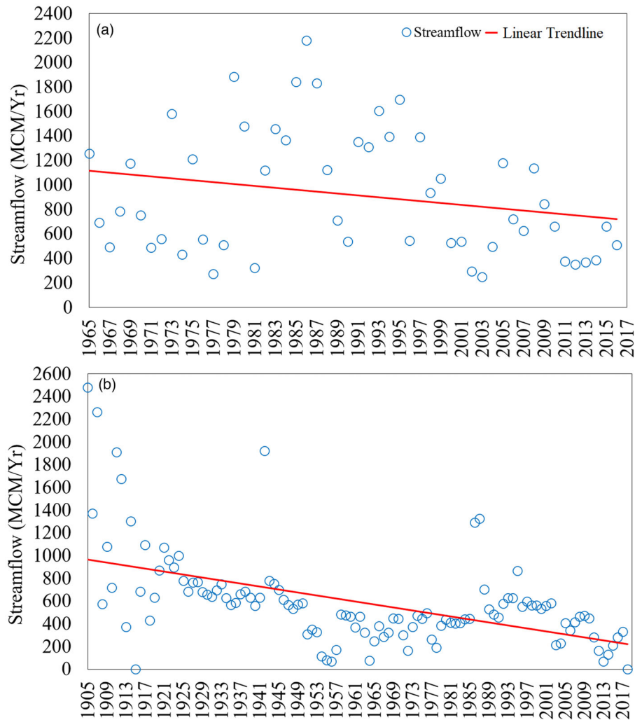
FIGURE 13. Historical annual variability of Rio Grande flow at (a) San Marcial gauge (USGS 08358300) immediately upstream of the watershed, and (b) watershed outlet at El Paso gauge (USGS 08364000).
