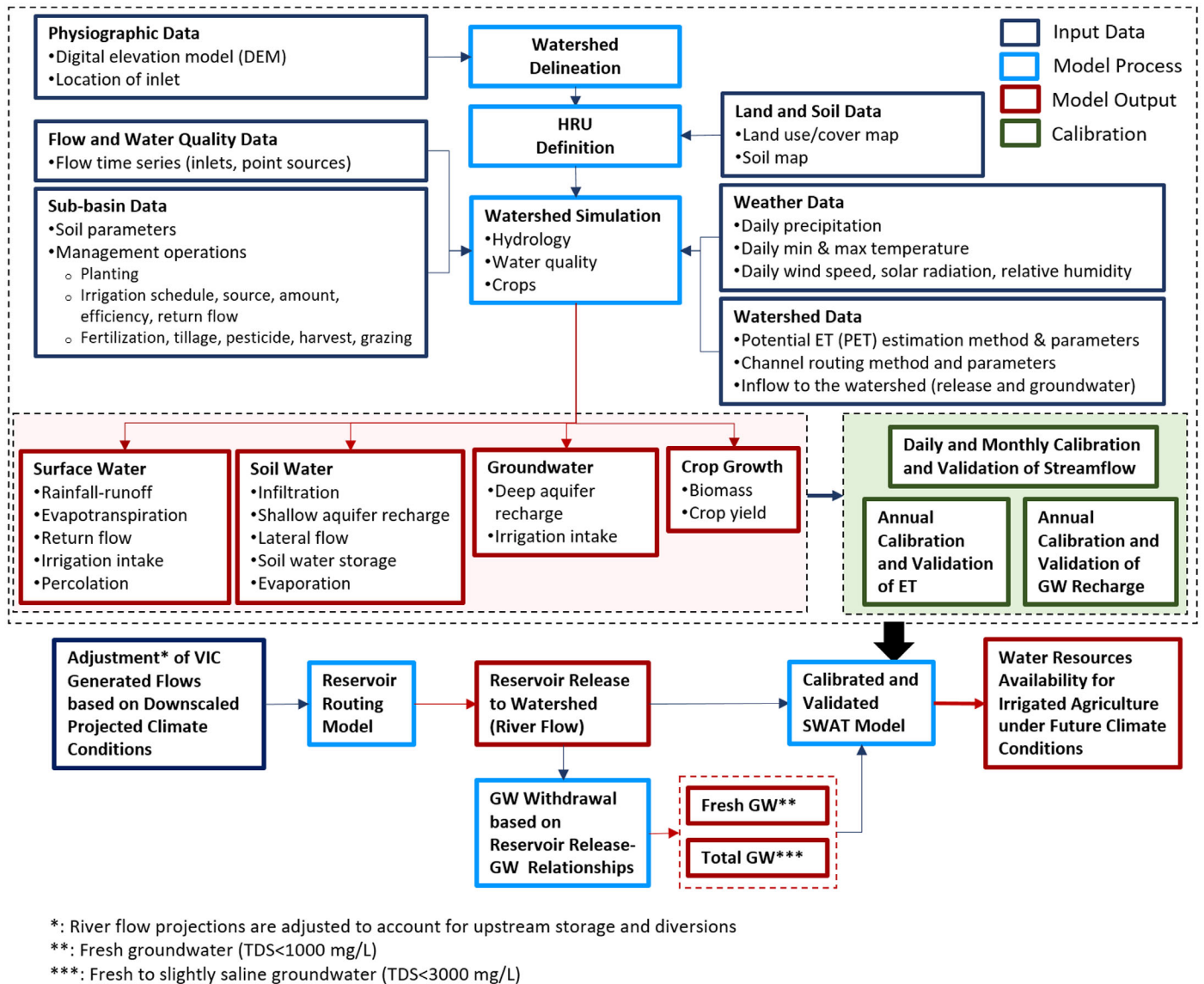
FIGURE 3. A general schematic of the climate impact assessment framework. ET, evapotranspiration; GW, groundwater; HRU, hydrological response unit; SWAT, Soil and Water Assessment Tool; VIC, variable infiltration capacity.
