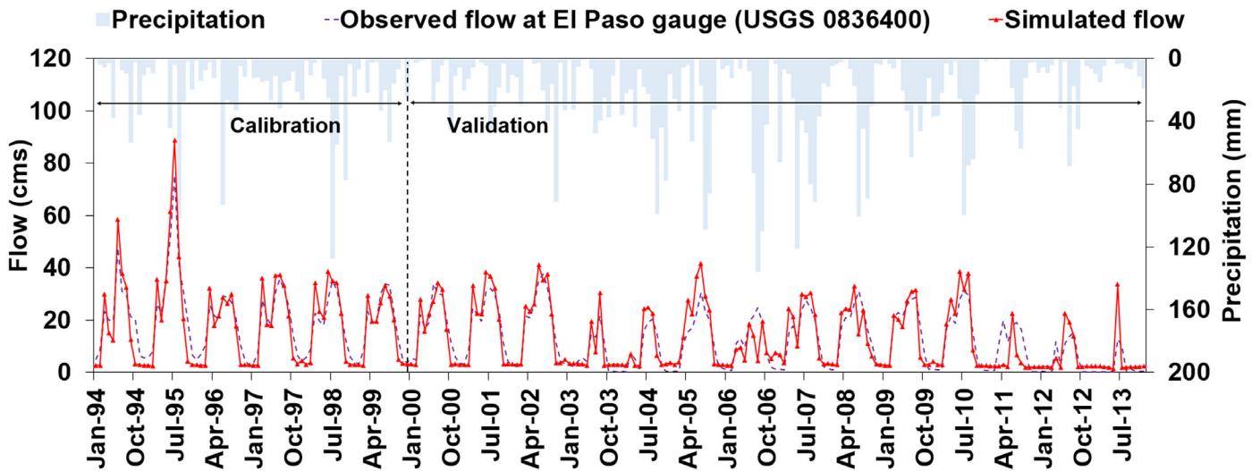
FIGURE 7. Comparison of observed streamflow with SWAT simulations.
