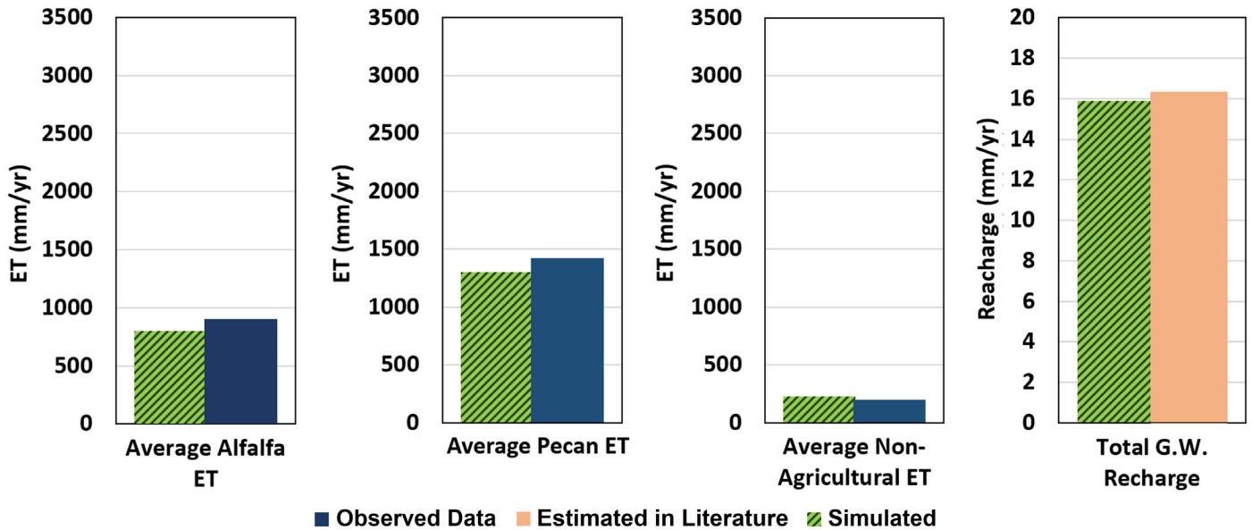
FIGURE 9. ET and groundwater recharge calibration compared with measured ET (Samani et al. 2004, 2013) and estimated recharge values in the Rincon Valley of Elephant Butte Irrigation District (Ahn et al. 2018).
