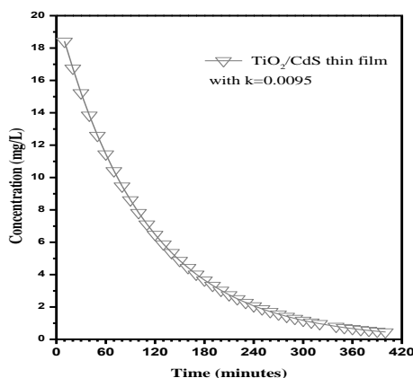
Fig. 10. Reaction kinetics of methylene blue degradation.
