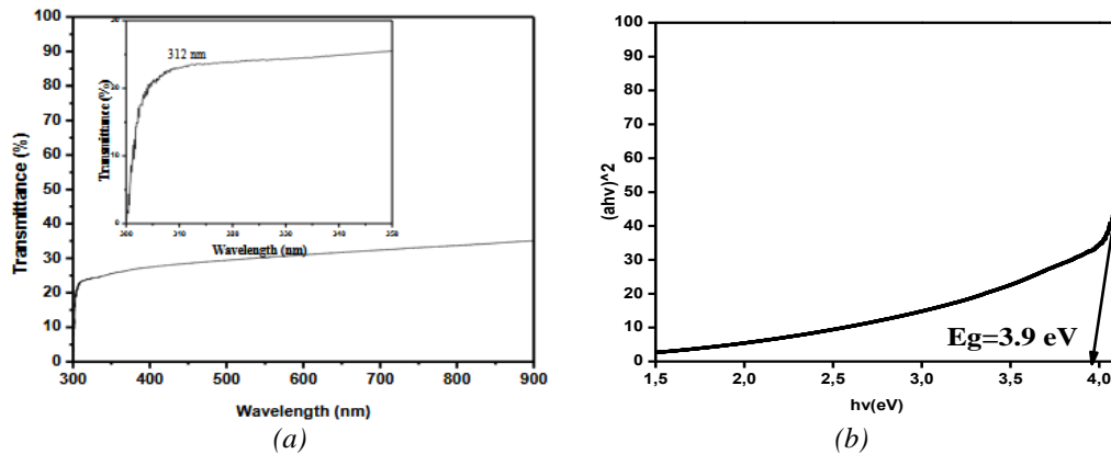
Fig. 4. (a) UV-Vis transmission spectra obtained for TiO 2 Nps thin film and (b) Tauc variable vs Energy.
