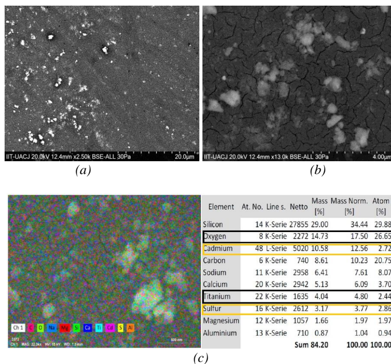
Fig. 8. (a) and (b) SEM micrographs and (c) EDAX analysis for \text{TiO}_2/\text{CdS} thin films.
