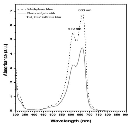
Fig. 9. Absorption spectrum of a solution of methylene blue concentration before and after of 60 minutes of heterogeneous photocatalysis.
