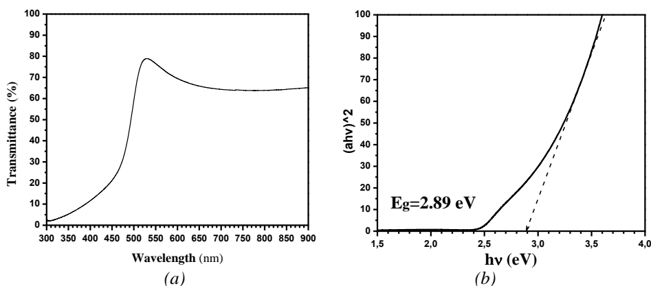
Fig. 1. (a) UV-Vis transmission spectra obtained for a CdS thin film deposited by CBD; (b) Tauc variable vs Energy.
