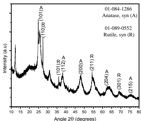
Fig. 6. XRD pattern for \text{TiO}_2 NPs. The planes corresponding to their corresponding reference code.
