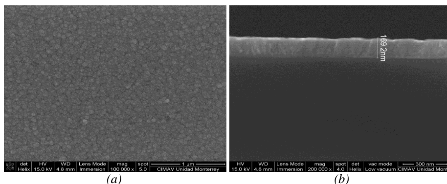
Fig. 2. SEM micrographs for CdS thin films deposited by CBD a) surface and b) cross-section.
