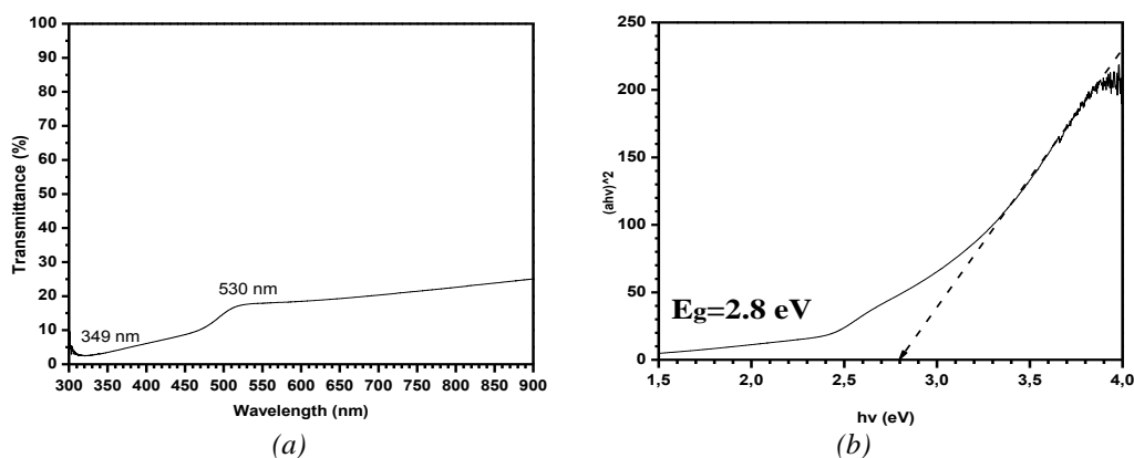
Fig. 7. a) UV-Vis transmission spectra for a \text{TiO}_2 NPs/CdS thin film, b) Tauc variable vs Energy.
