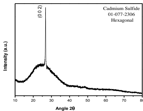
Fig. 3. XRD pattern for CdS thin films by CBD.
