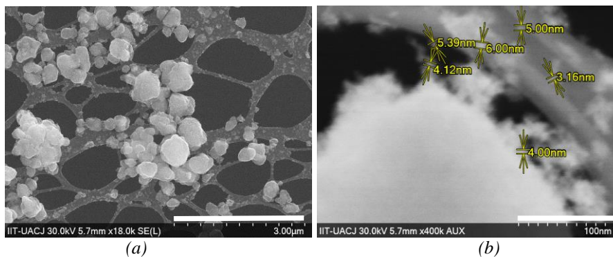
Fig. 5. SEM micrographs for TiO 2 nanoparticles.
