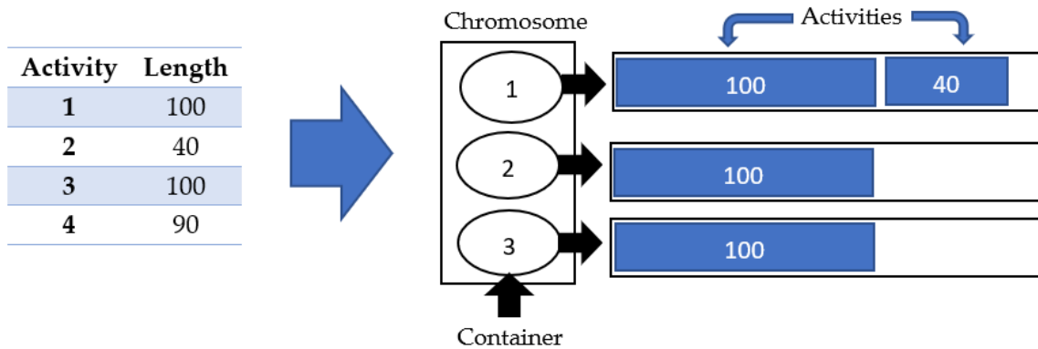
Figure 1. Genetic coding.
