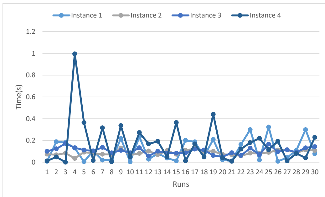
Figure 12. Execution time.
